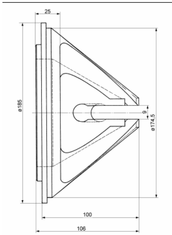
Nose Cone M5K P02
