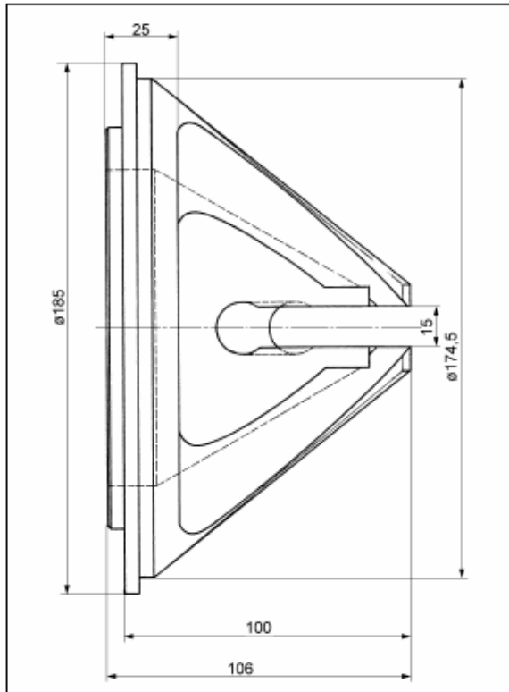
Nose Cone M5K P01
